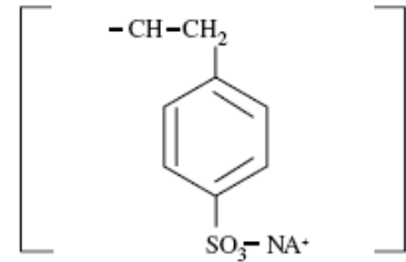
Figure 1 Sulfonated Polystyrene
