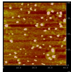
Figure 2. AFM image of annealed P3HT/PCBM on top of PEDOT and Silicon. There is noticeable phase separation and uniformity of the PCBM aggregates.
