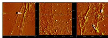
Figure 2: Examining fiber growth through AFM scans (contact mode): PS (left), PMMA (Mid), PMMA/PS blend (Right).
