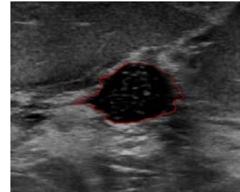
Figure 2: Segmented Image
